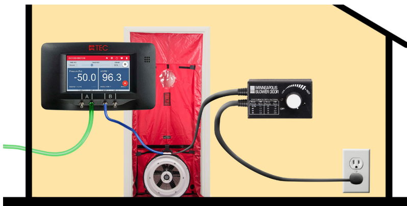
Figure 4. How blower door components are connected.
